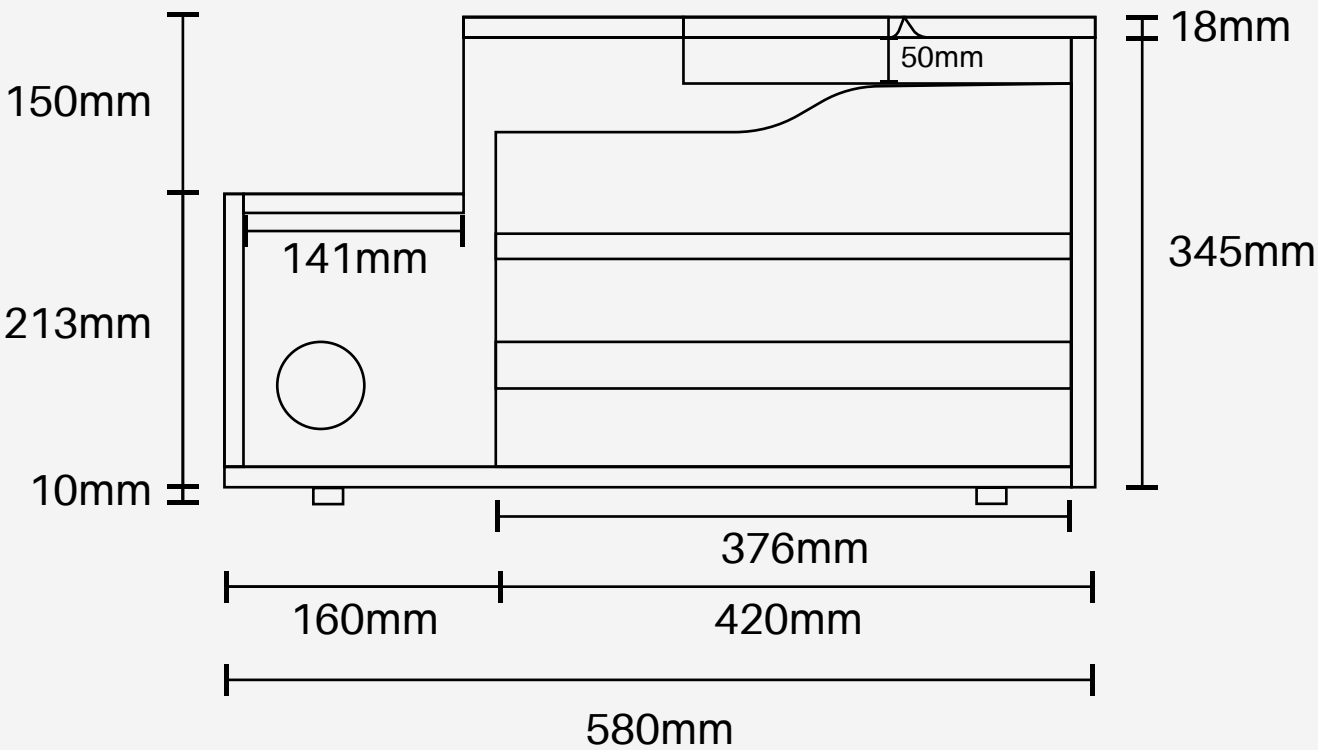
Left Side View: Internal dimensions of the middle cabinet
