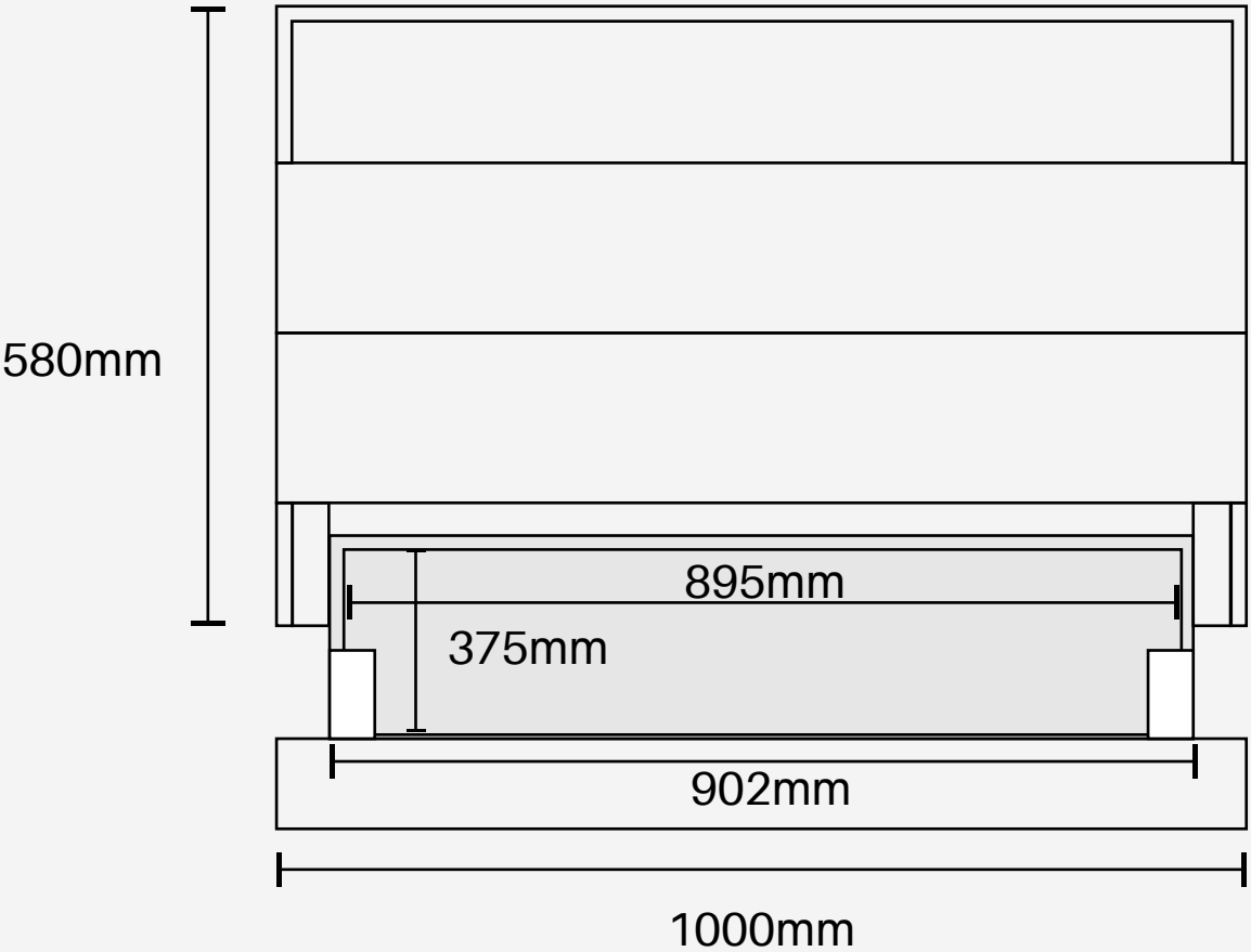
view from above: the maximum move distance of motorised drawer
